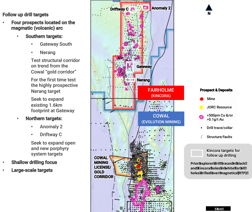
Figure 7: Four large-scale prospects identified for follow up drilling Kincora will shortly own a 100% interest in the Fairholme project
