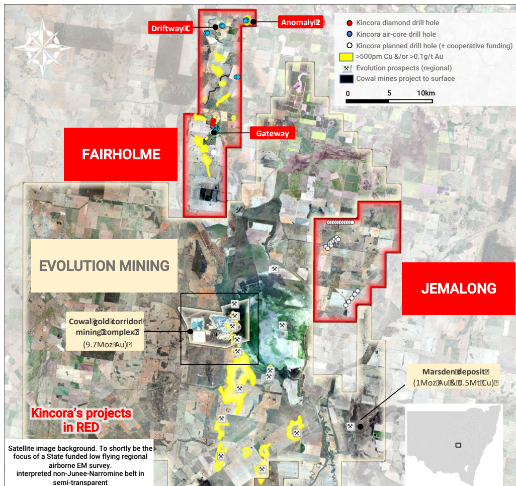
Figure 4: Fairholme – On mineralised trend and adjacent to the Cowl “gold corridor” and mine The wider Cowl project hosts a 14Moz gold and 0.5Mt copper endowment
